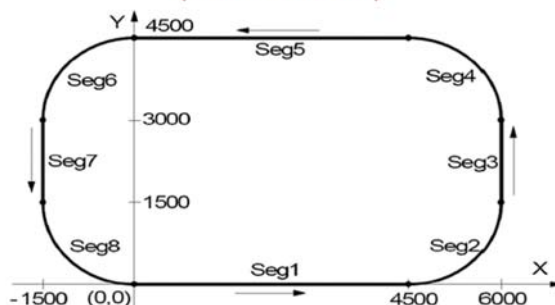
Continuous interpolation
