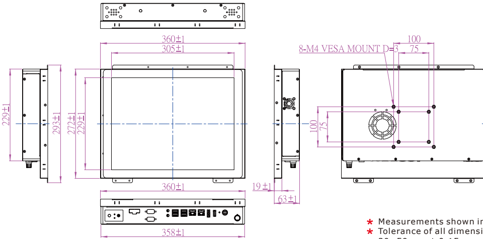
Modularized Construction Dimensions
