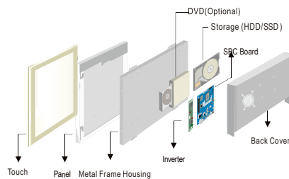
Mechanical design
