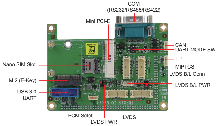
IBR215-I/O (Option)
