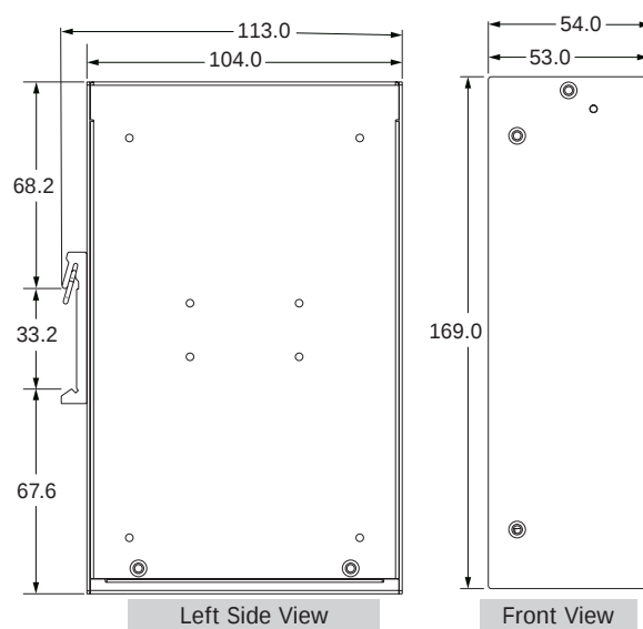
USB-4018HS-16
