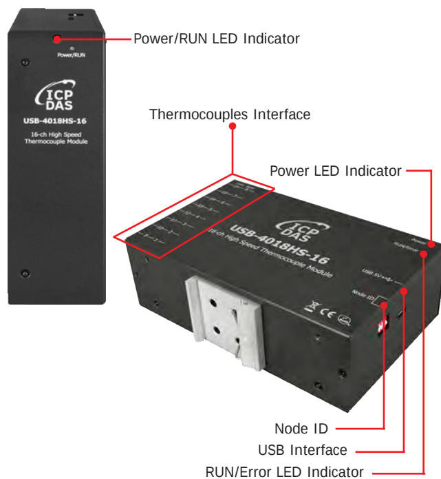
USB-4018HS-16
